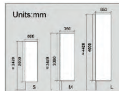
Indoor Flag Pole Dimensions
